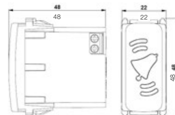
Campainha cigarra
