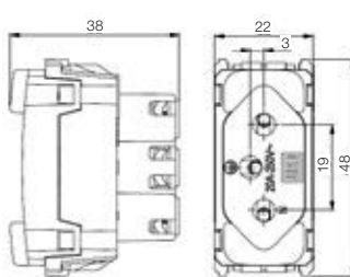
Tomada 2P+T-20 A
