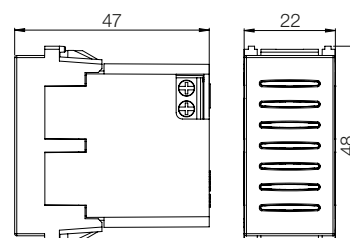
Campainha cigarra
