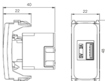
Tomada USB Keystone
