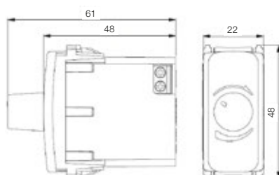
Dimmer
